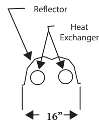
-End View-
